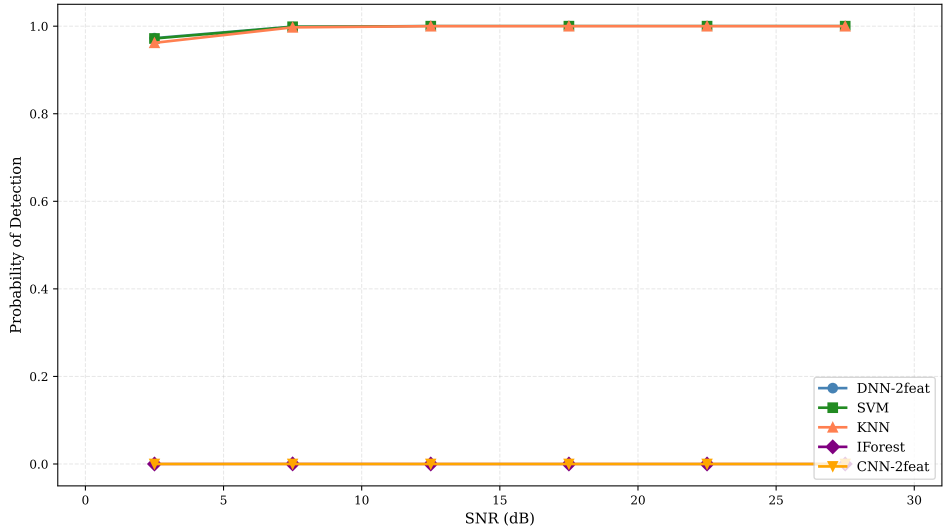
P_D vs SNR ( \alpha = 10^{-7} )
